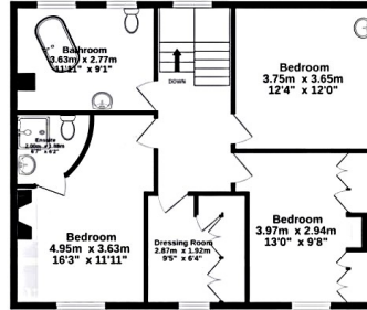
1st Floor 70.4 sq.m. (757 sq.ft.) approx.
