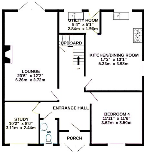
GROUND FLOOR 950 sq.ft. (88.3 sq.m.) approx.
