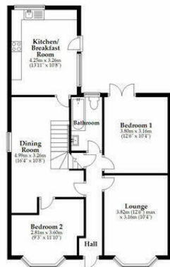
Ground Floor Approx. 143.7 sq. metres (1546.7 sq. feet)
